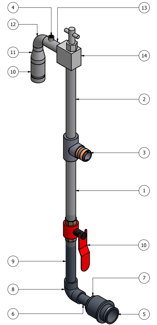
CW-SP-001 1 1/4" SS CONCENTRATE OUT
