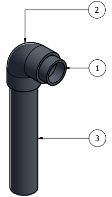
CIP-PP-001 2" FEED OUTLET FROM TANK (INSIDE TANK)
