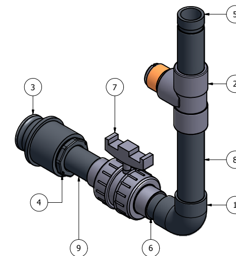
PW-PP-002 1 1/4" PERMEATE PIPE
