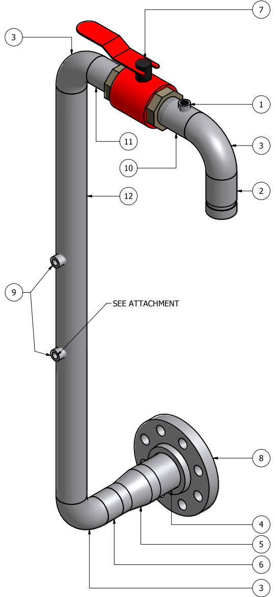
FW-SP-001 RO 1 1/2" SS FEED
