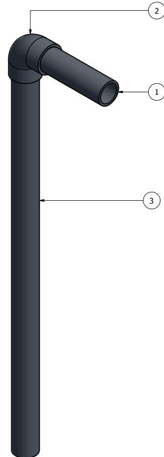
PR-PP-001 2" PERMEATE RETURN (INSIDE TANK)
