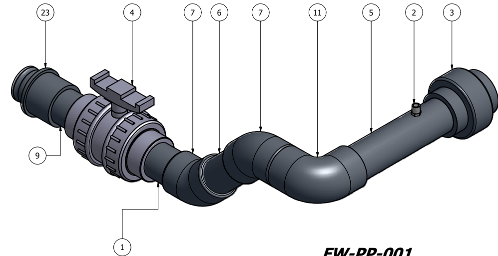
FW-PP-001 2" PVC MAIN FEED
